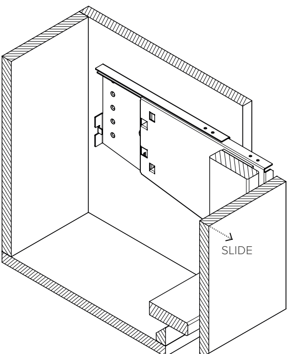
4. Slide out spring boxes from metal boxes.
