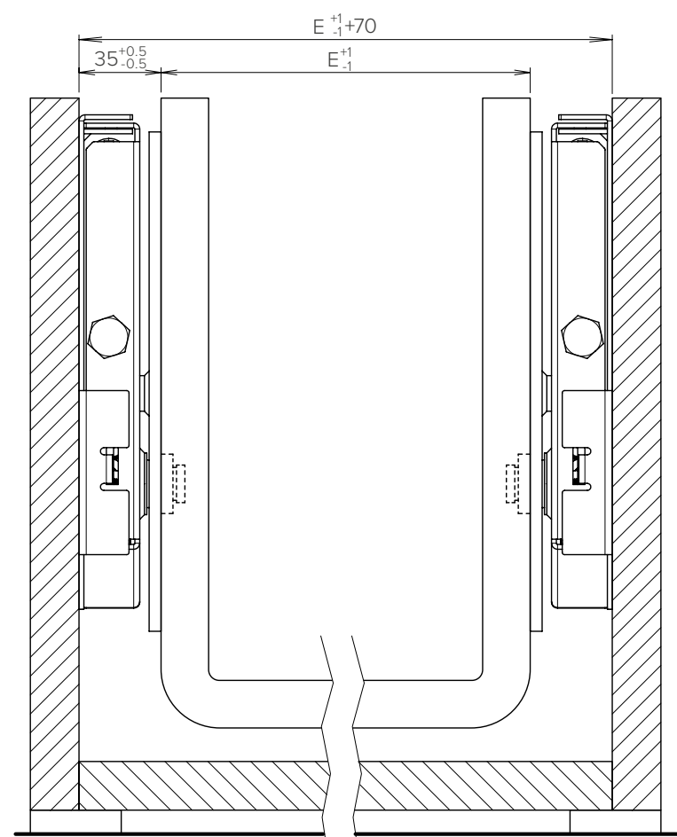
Reference dimensions to build the cabinet
