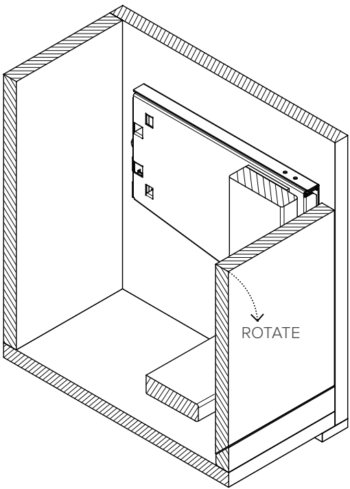
1. Rotate the mechanism in horizontal position.
